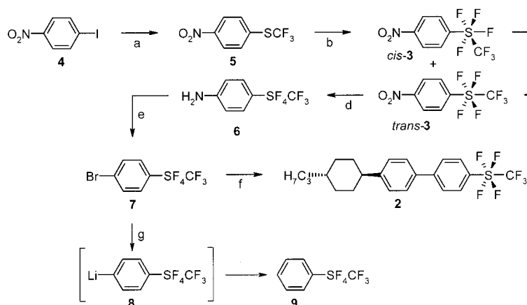
Scheme 2. Synthesis of the liquid crystal 2 and [trans-(trifluoromethyl)tetrafluorosulfuranyl]benzene ( 9 ): a) CuSCF 3 , DMF; 130 °C (60%). b) 10% F 2 /N 2 , CH 3 CN; –3–2 °C (50% of a cis / trans , 85:15 mixture). c) AlCl 3 (0.8 equiv.), CH 2 Cl 2 ; –10 °C, 30 min (48% pure trans ). d) Cat. Raney-Ni, H 2 , THF; room temp., 1 bar (87%). e) 1. NaNO 2 , 47% HBr; 0–5 °C; 2. CuBr; 85 °C (52%). f) 4-( trans -4-propylcyclohexyl)-benzeneboronic acid, NaBO 2 ·8H 2 O, H 2 O, THF, cat. Pd(PPh 3 ) 4 ; 60 °C, 5 h (14%). g) 1. tert -BuLi, Et 2 O; –70 °C, 1.5 h; 2. H 2 O; –70 °C → room temp. (11%).
